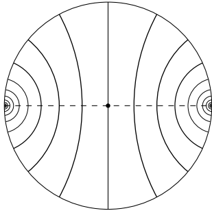
FIGURE 4. Images of the imaginary axis under some powers of the translation \begin{pmatrix} 4/\sqrt{15} & 1/\sqrt{15} \\ 1/\sqrt{15} & 4/\sqrt{15} \end{pmatrix} .
