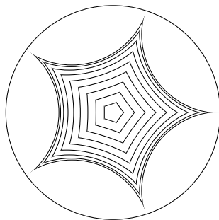
(B) Hyperbolic geodesic pentagons.
