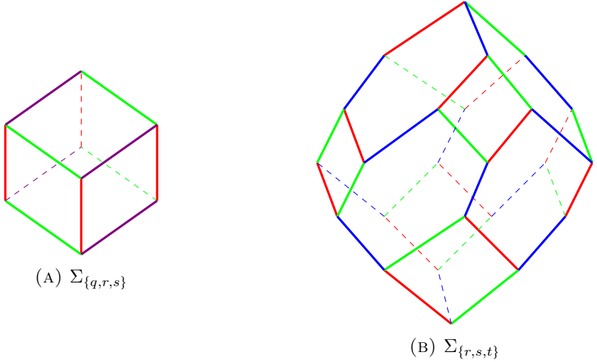
FIGURE 4. Coxeter cells for Example 2.3.6.
