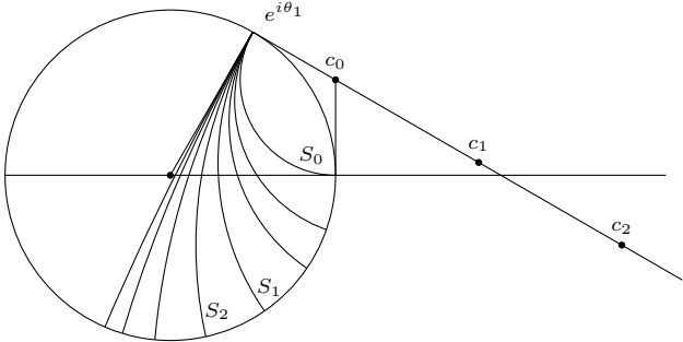
FIGURE 6. Construction of a geodesic with angle \theta_2 and endpoint at e^{i\theta_1} .
