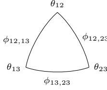
(B) The link of vertex v .
