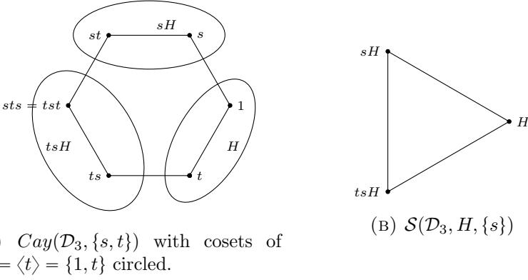
FIGURE 1. A Cayley graph and coset graph for \mathcal{D}_3 .
