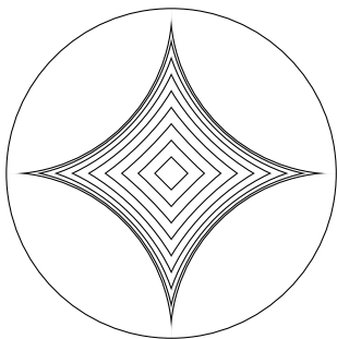
(A) Hyperbolic geodesic squares.
