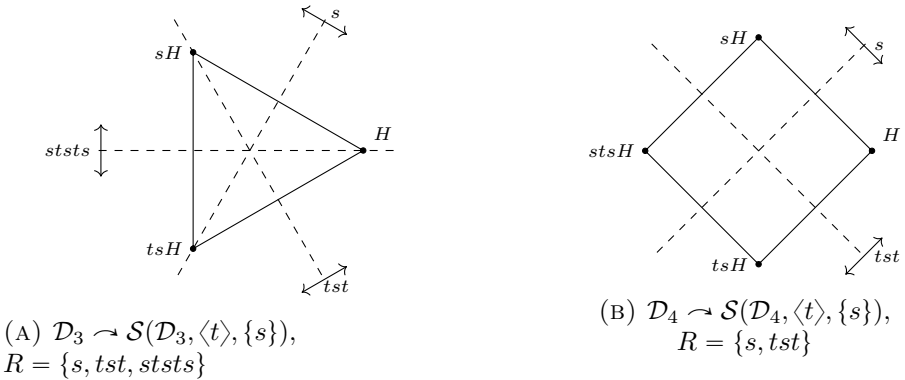
FIGURE 2. Two examples of \mathcal{D}_m acting on one of its simple coset graphs. The m = 3 case is a prereflection system, but the m = 4 case is not, because in that case R does not generate \mathcal{D}_4 .
