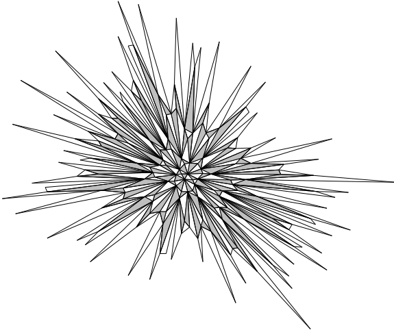
(A) Part of the Coxeter complex of \Delta(5, 5, 2) in V^* , viewed from (1, 1, 1) .
